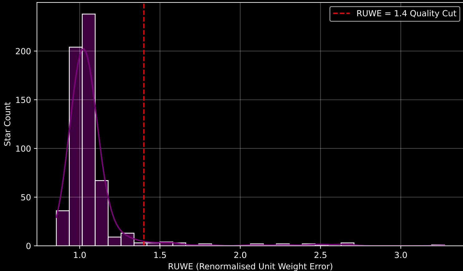
GAPOGEE DR17 Field [030+08] RUWE Distribution (n= 593)
