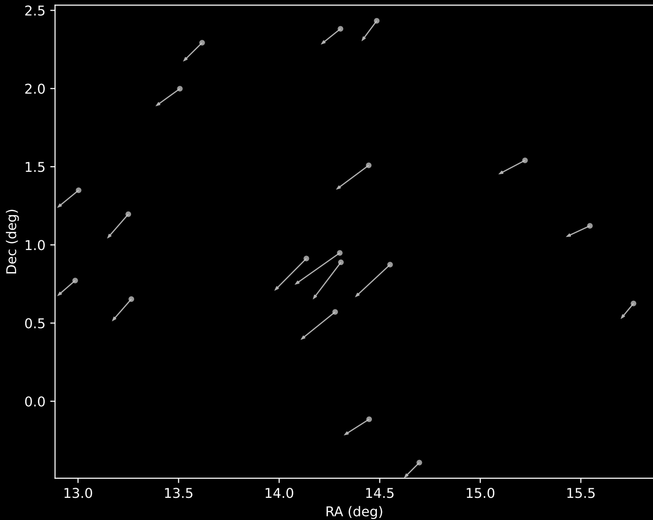
APOGEE DR17 Cluster 15 Proper Motion Vectors (n=19)
