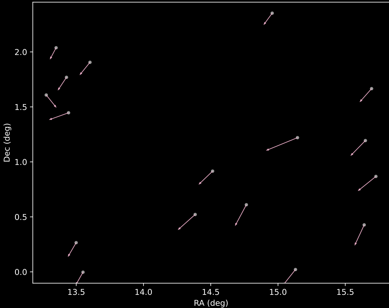
APOGEE DR17 Cluster 13 Proper Motion Vectors (n=17)
