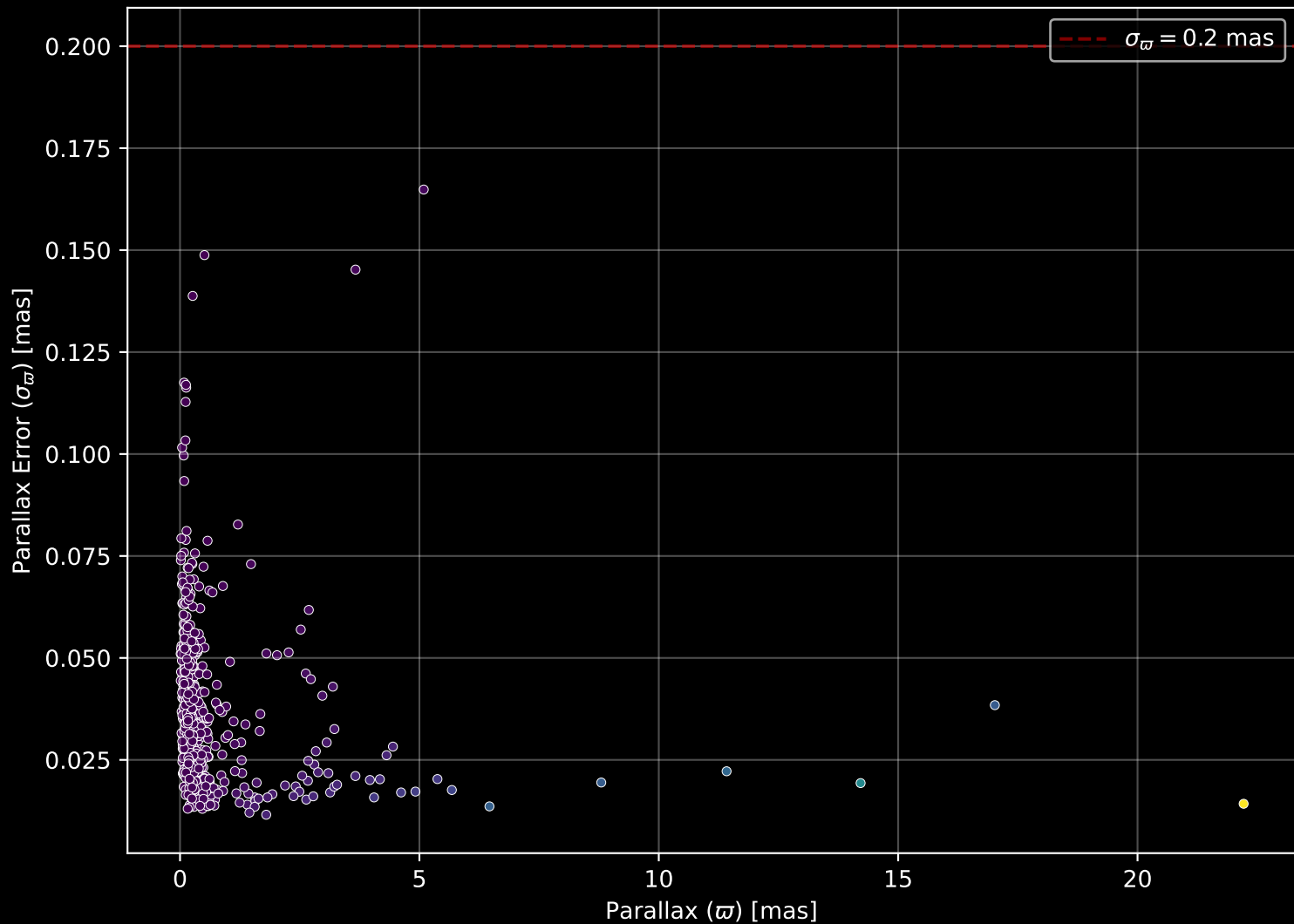
APOGEE DR17 Field: [030+08] Parallax Quality (n= 596)
