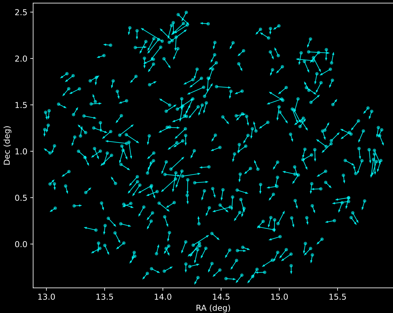
APOGEE DR17 Noise Stream Proper Motion Vectors (n=311)
