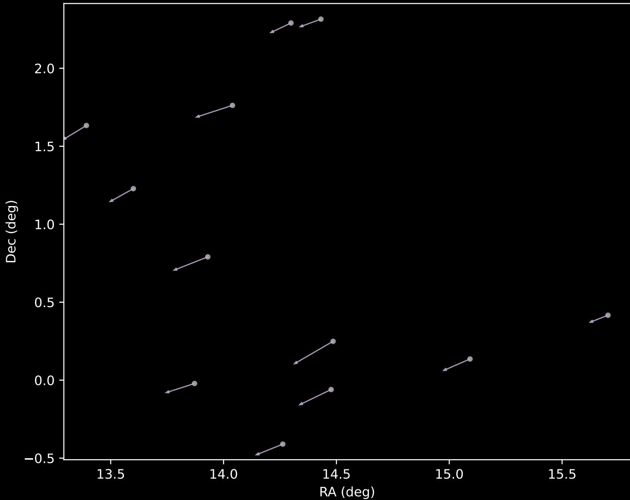
APOGEE DR17 Cluster 9 Proper Motion Vectors (n=12)
