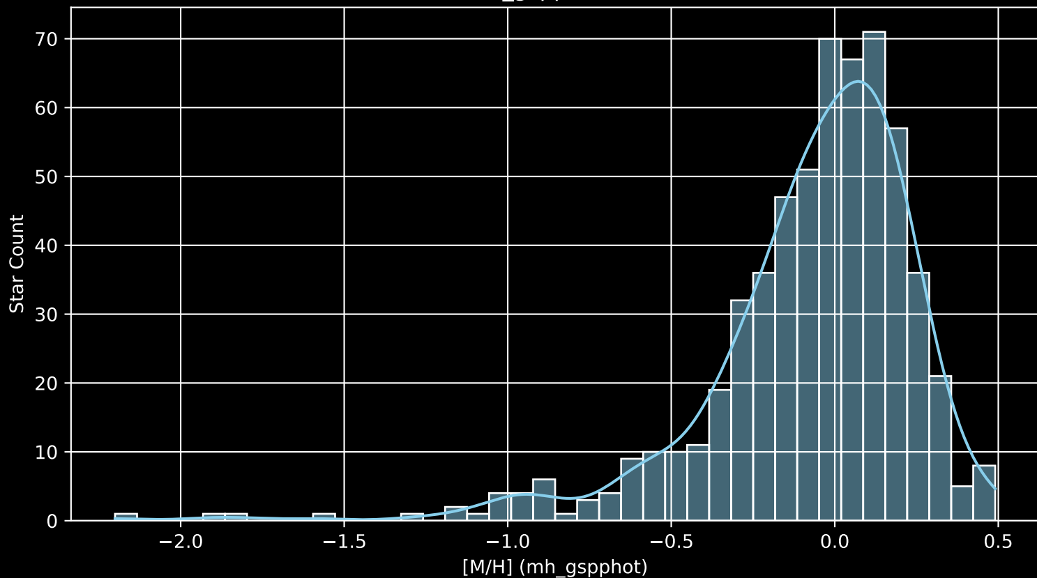
APOGEE DR17 Field: [030+08 [M/H] (mh_gspphot) (n= 590)
