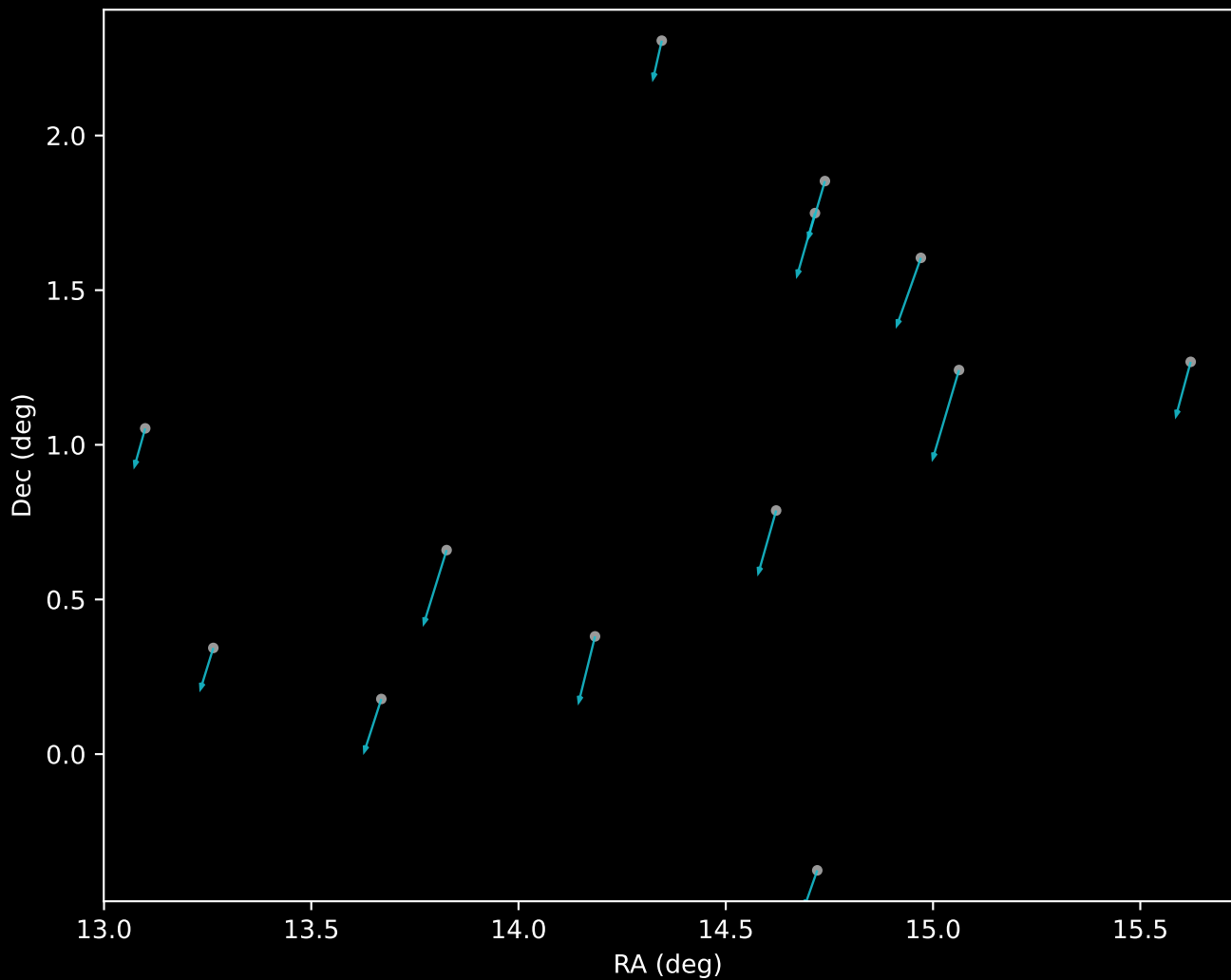
APOGEE DR17 Cluster 18 Proper Motion Vectors (n=13)
