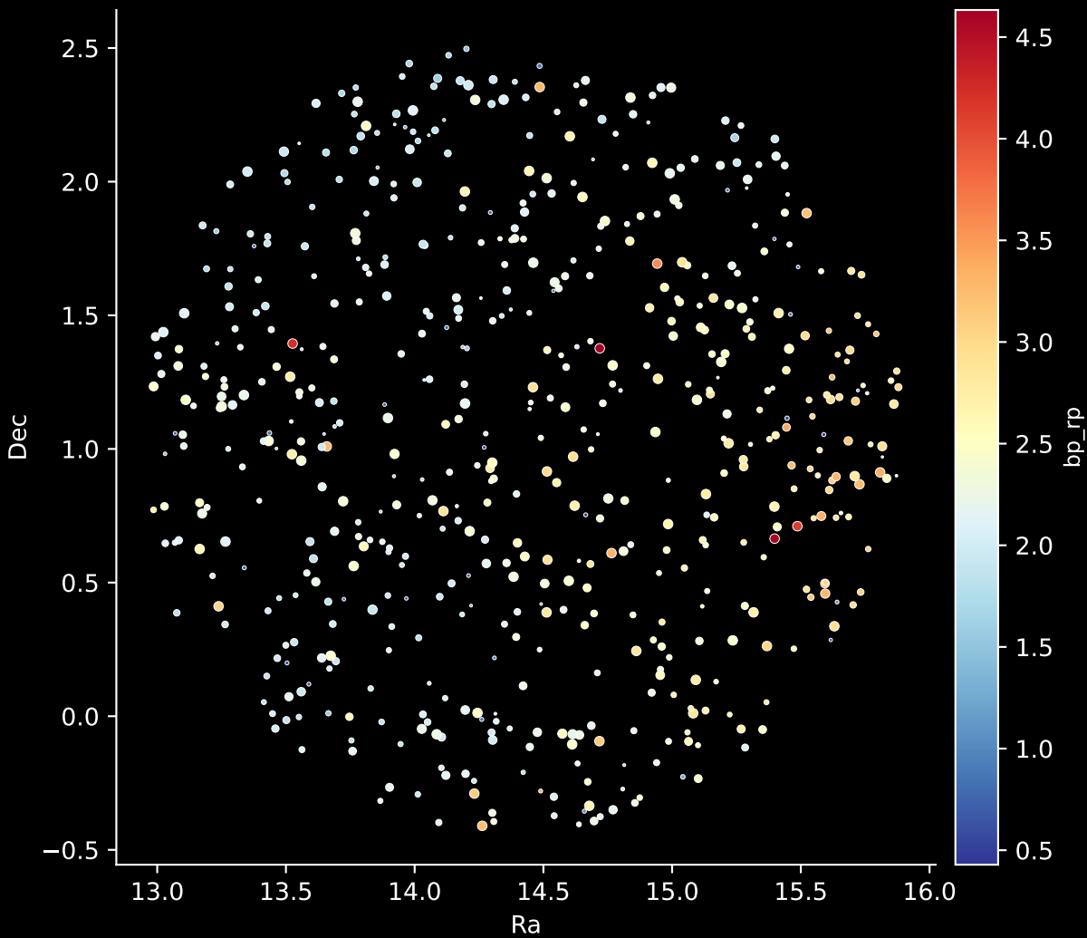
APOGEE DR17 Field: [030+08] Stars: 596
