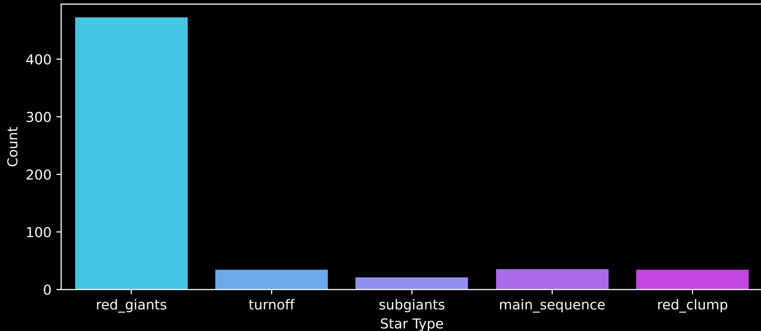
APOGEE DR17 Field: [030+08] Count plot of Star Type
