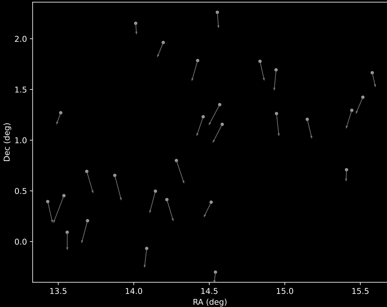
APOGEE DR17 Cluster 14 Proper Motion Vectors (n=28)
