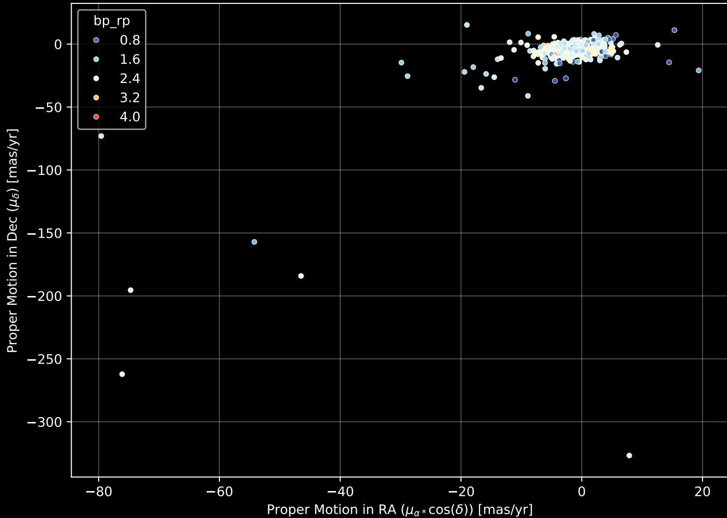
APOGEE DR17 Field: [030+08] Proper Motion Diagram (n= 596)
